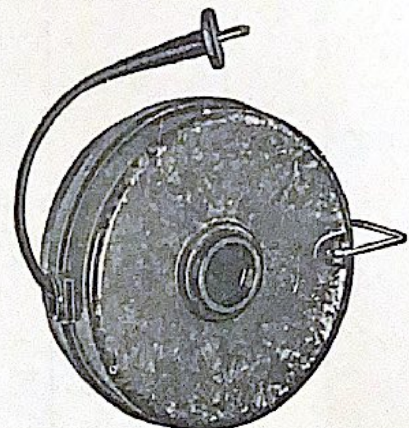
Stromfix Senior (1760)
